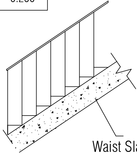
Staircase Details
