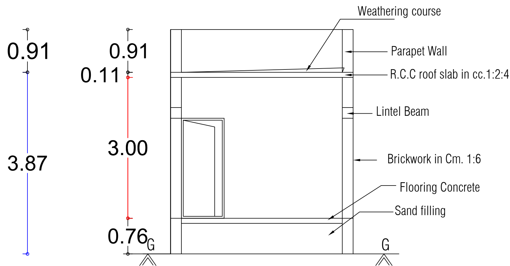
FRONT ELEVATION
