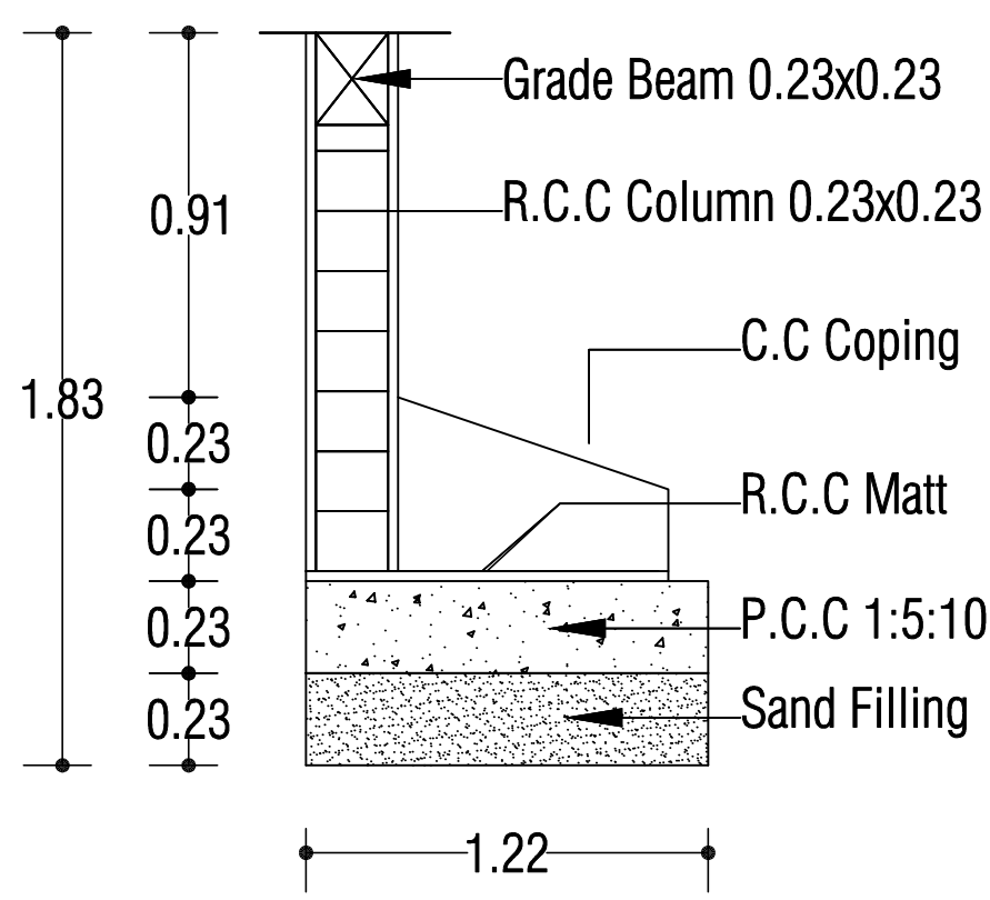
Foundation Details
