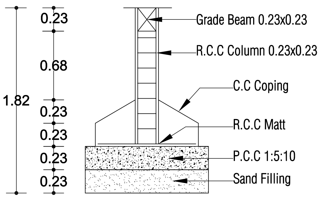
Foundation Detail
