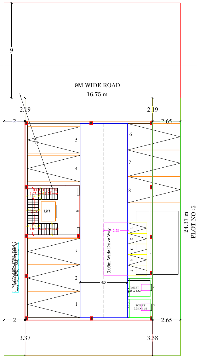
SITE CUM STILT FLOOR PLAN
