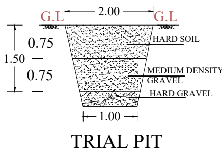
TRIAL PIT
