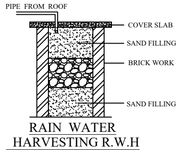
RAIN WATER HARVESTING R.W.H
