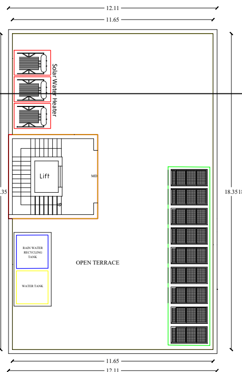
TERRACE PLAN
