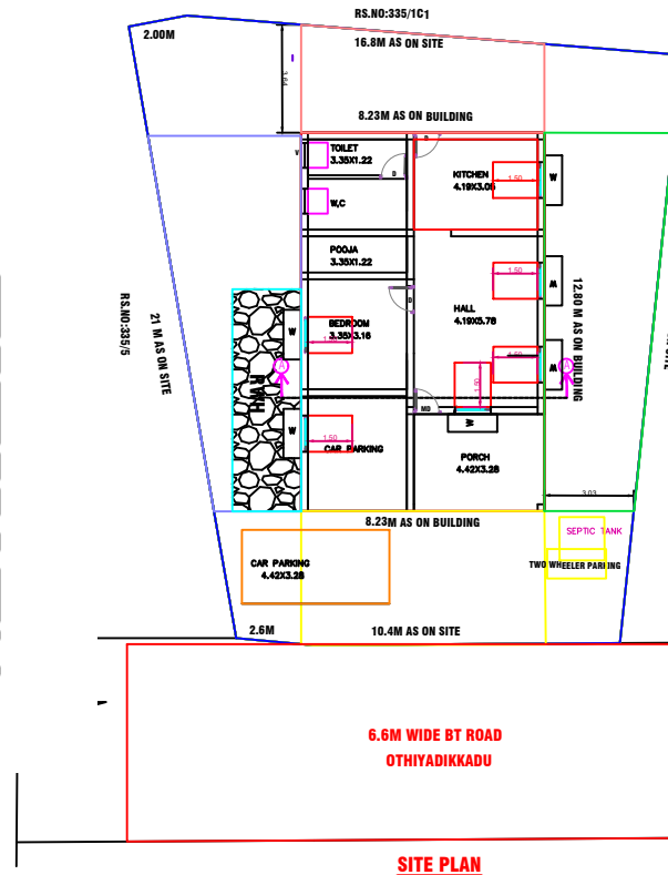
SITE PLAN
