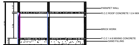
CROSS SECTION
