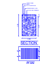
RAIN WATER HARVESTING PERCOLATION BED
