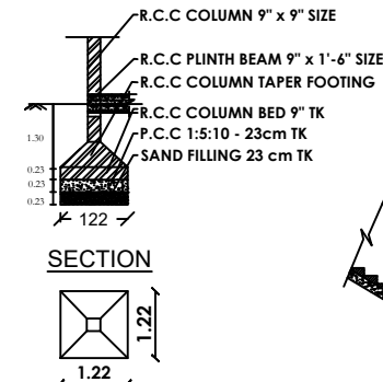
COLUMN DETAILS PLAN
