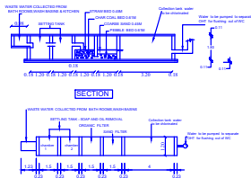
WASTE WATER RECYCLING SYSTEM
