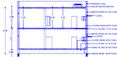
SECTION ON A-A1
