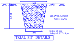
TRIAL PIT DETAILS
