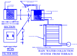
RAIN WATER COLLECTION SYSTEM FROM TERRACE
