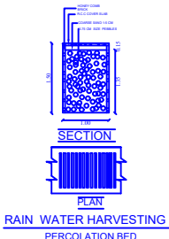
RAIN WATER HARVESTING PERCOLATION BED
