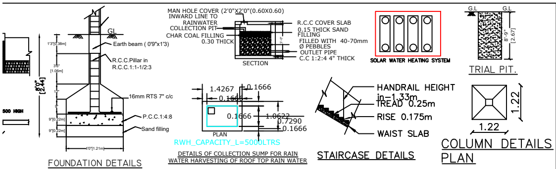
FOUNDATION DETAILS
