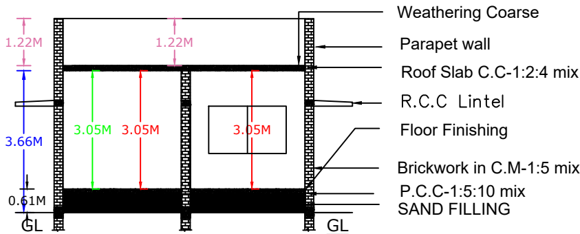
SECTION ON XX
