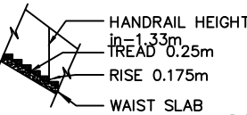
STAIRCASE DETAILS
