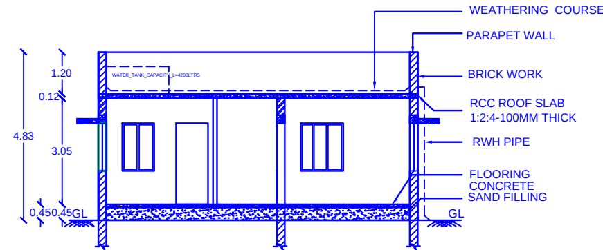
SECTION X-Y
