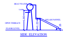
SIDE ELEVATION
