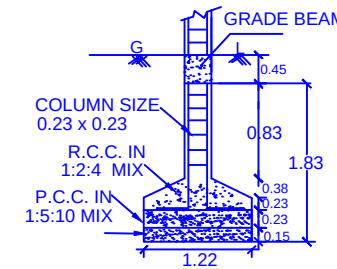
COLUMN DETAILS SCALE 1:25
