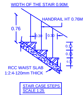
STAIR CASE STEPS SCALE 1:25
