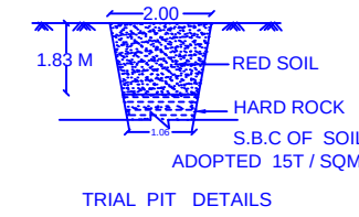
TRIAL PIT DETAILS SCALE 1:25
