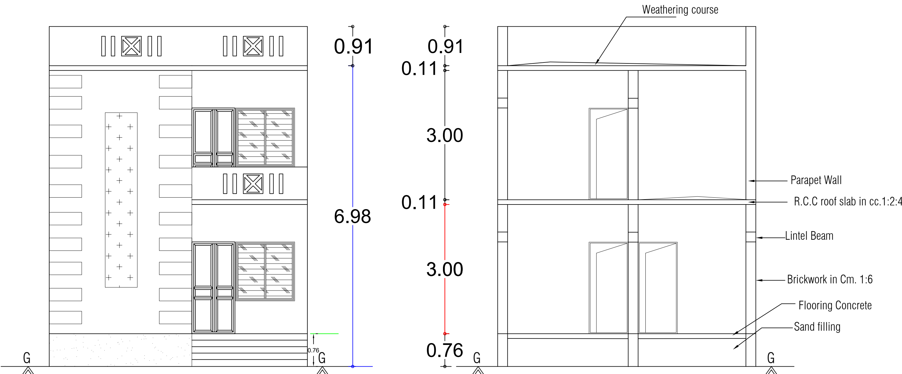
FRONT ELEVATION
