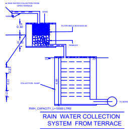
RAIN WATER COLLECTION SYSTEM FROM TERRACE
