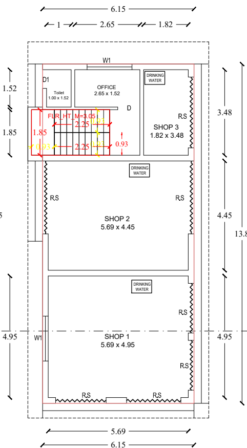
EXI-GROUND FLOOR PLAN
