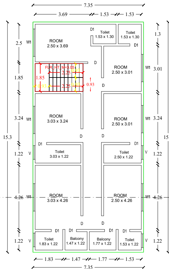
EXI-FIRST FLOOR PLAN
