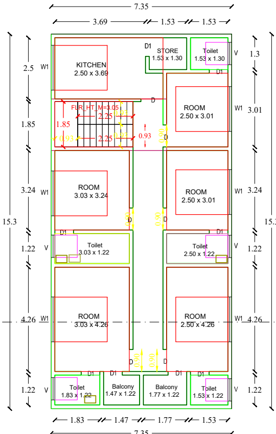
PRO-THIRD FLOOR PLAN
