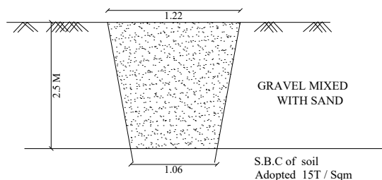
TRIAL PIT DETAILS
