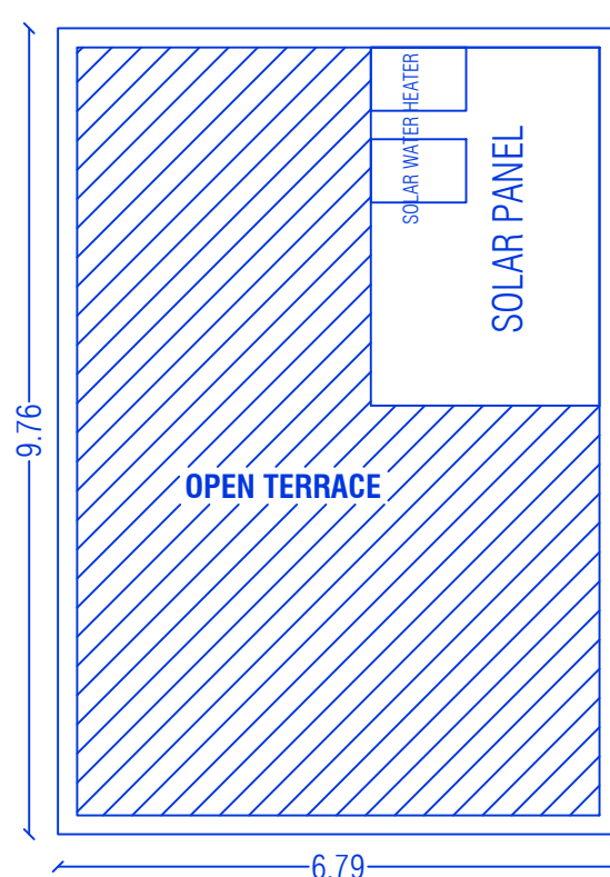
TERRACE PLAN
