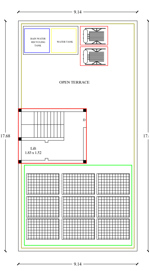
TERRACE PLAN
