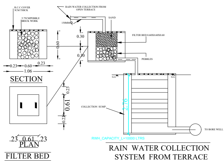
RAIN WATER COLLECTION SYSTEM FROM TERRACE
