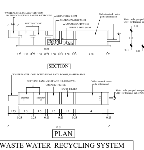
WASTE WATER RECYCLING SYSTEM
