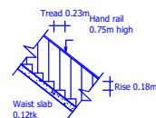
STAIR DETAILS
