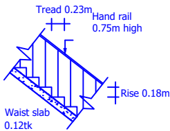
STAIR DETAILS
