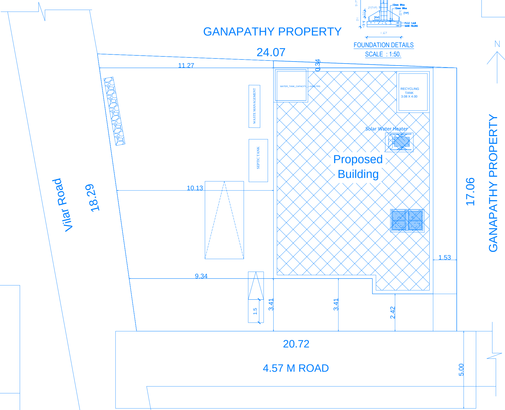
SITE PLAN
