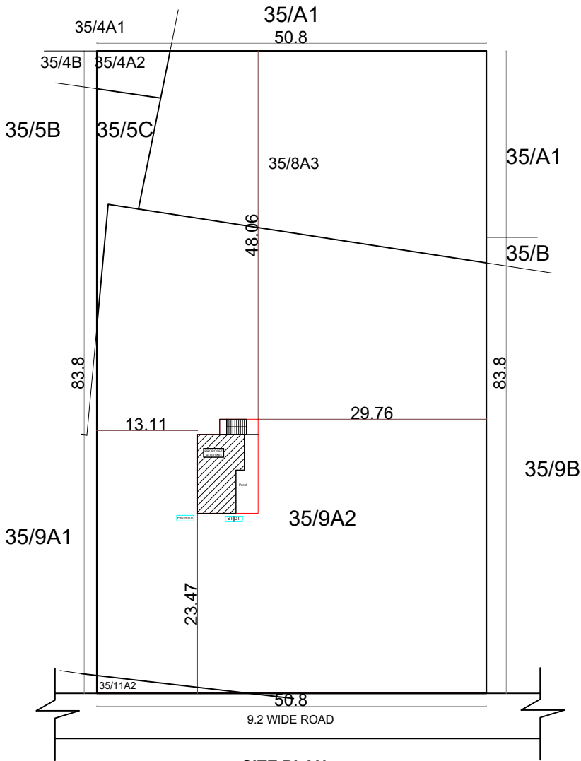
SITE PLAN
