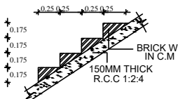
STAIRCASE DETAILS
