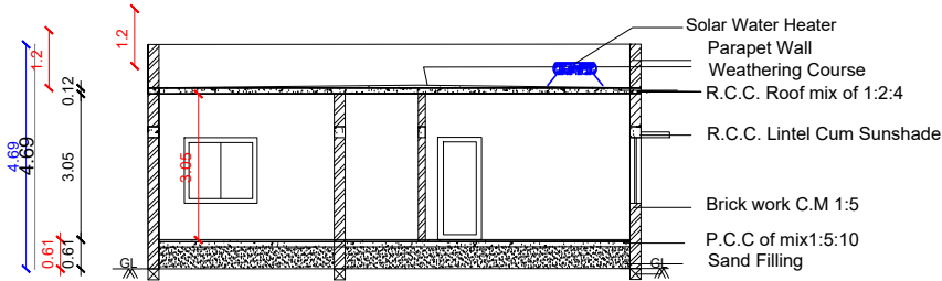
SECTION ON RR
