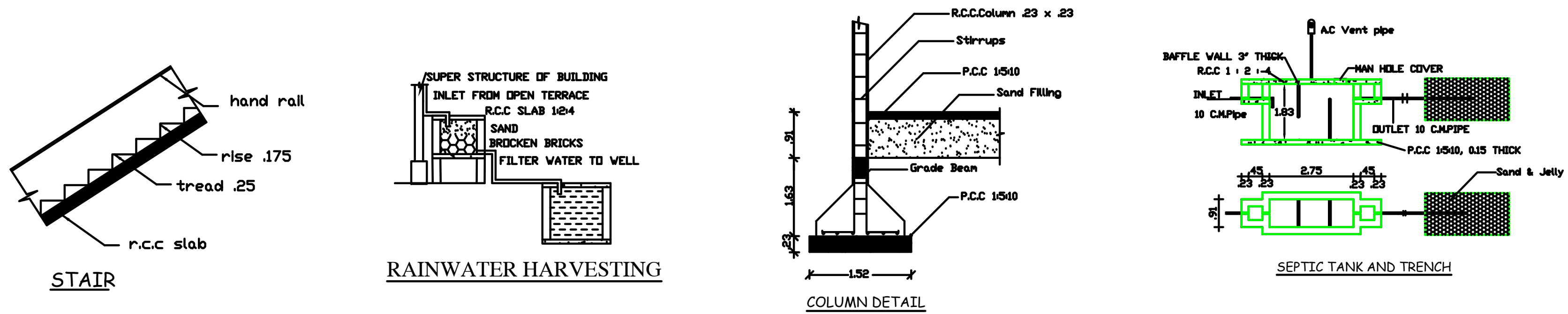
COLUMN DETAIL
