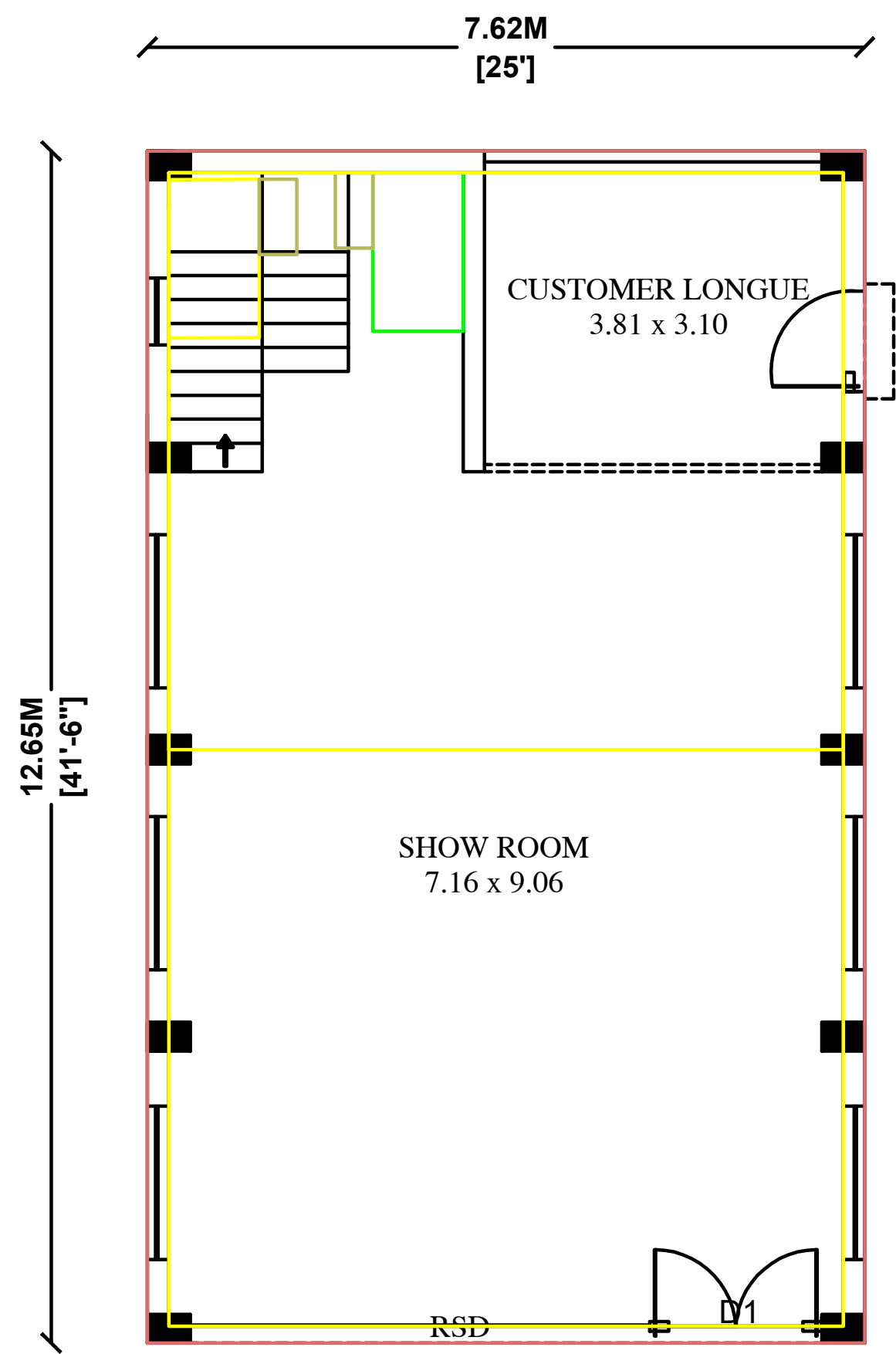
PRO.GOUND FLOOR PLAN
