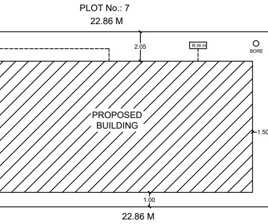
SITE PLAN
