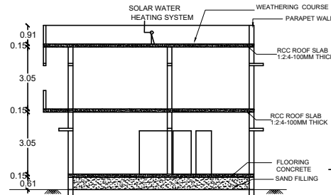
SECTION NP
