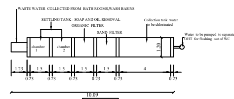
WASTE WATER RECYCLING SYSTEM
