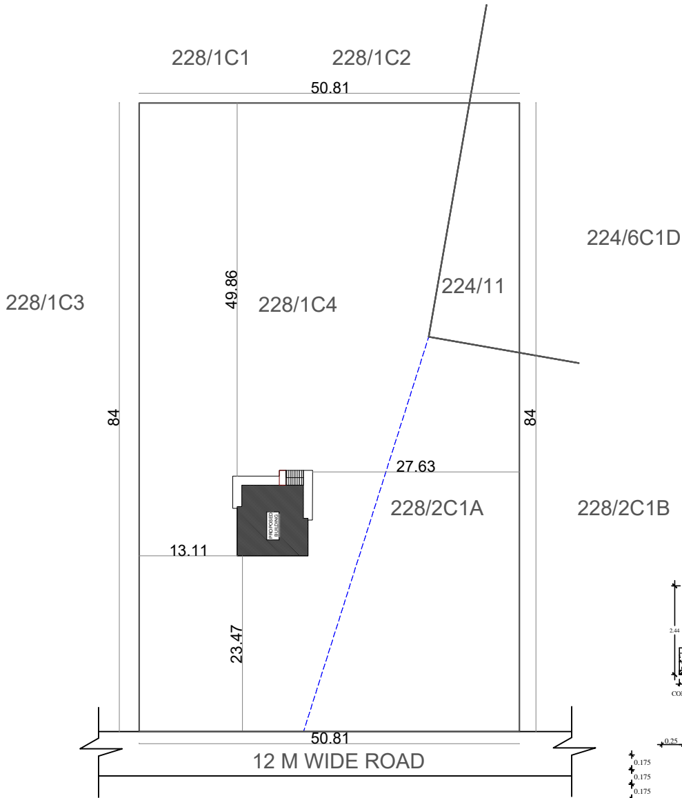
SITE PLAN
