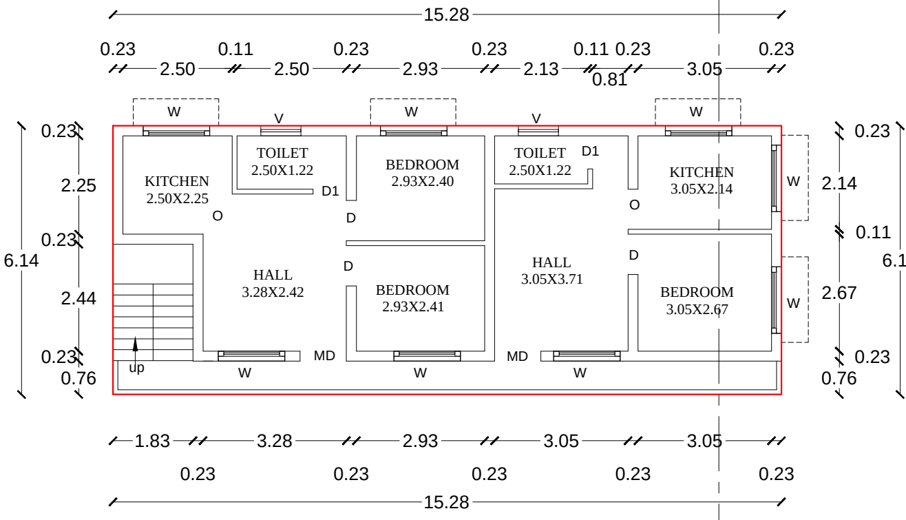
PRO- SECOND FLOOR PLAN
