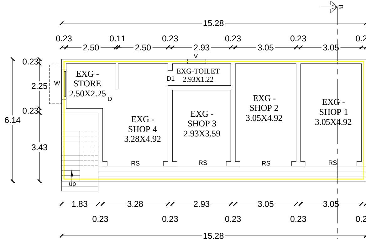
EXG- GROUND FLOOR PLAN
