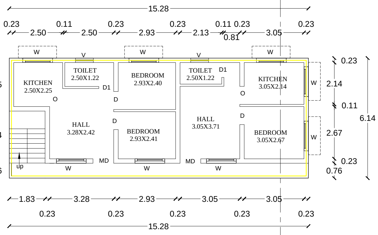
EXG- FIRST FLOOR PLAN
