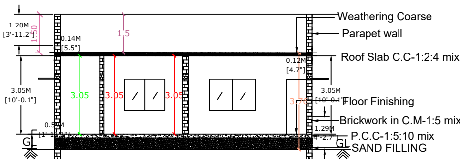
CROSS SECTION ON XX
