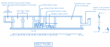
RAIN WATER HARVESTING PERCOLATION BED
