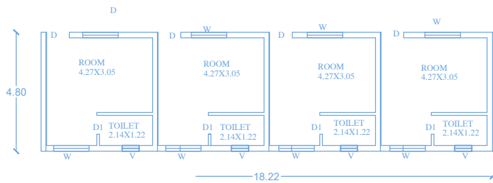
ND FLOOR PLAN
