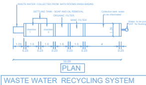
WASTE WATER RECYCLING SYSTEM
