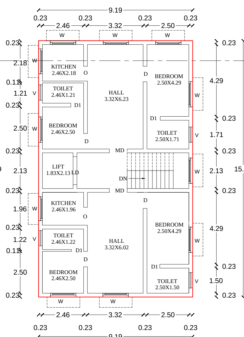
PRO- SECOND FLOOR PLAN
