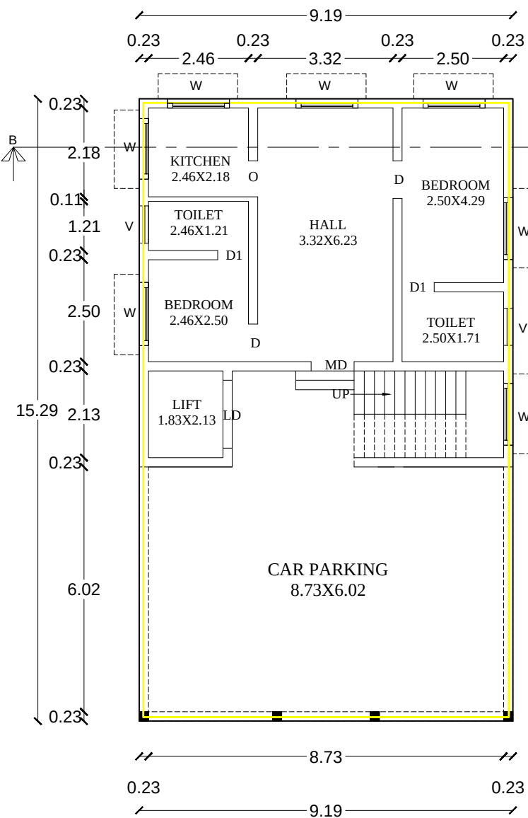
EXG- GROUND FLOOR PLAN
