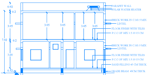
SECTION ON A-A1
