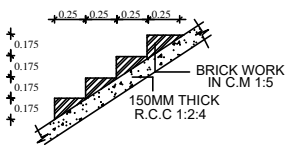
STAIRCASE DETAILS
