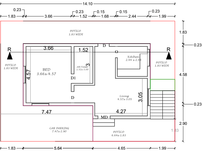
Prop Ground Floor
