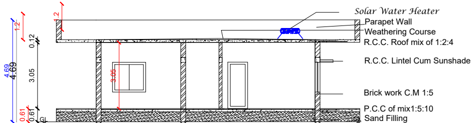
SECTION ON RR
