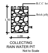
COLLECTING RAIN WATER PIT
