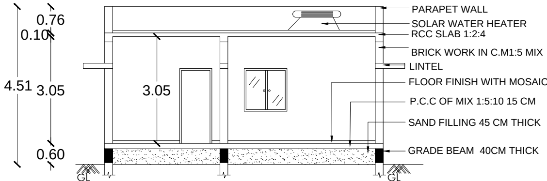
SECTION ON - 'RM'
