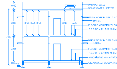
SECTION ON A-A1
