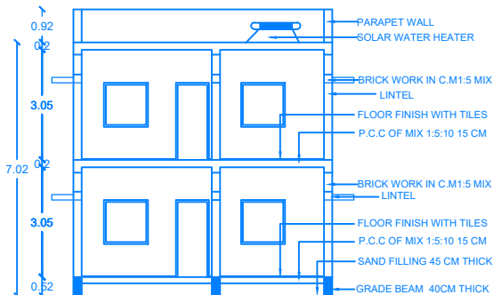
SECTION ON A-A1
