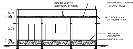
SECTION NP
