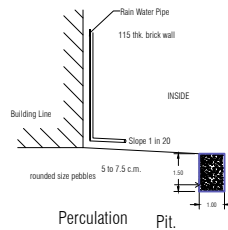
WATER HARVESTING
