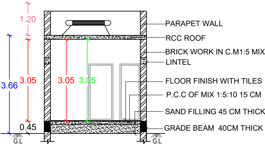
SECTION-AA1
