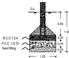
TRIAL PIT
