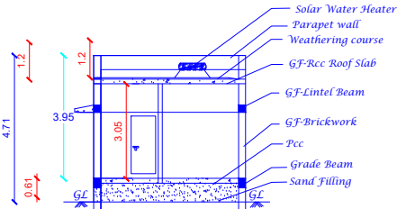
SECTION ON RR
