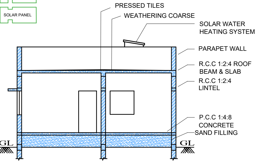
SECTION "A-B"
