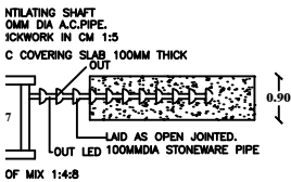
SEPTIC TANK
