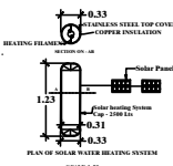
PLAN OF SOLAR WATER HEATING SYSTEM
