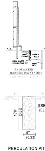
PERCOLATION PIT
