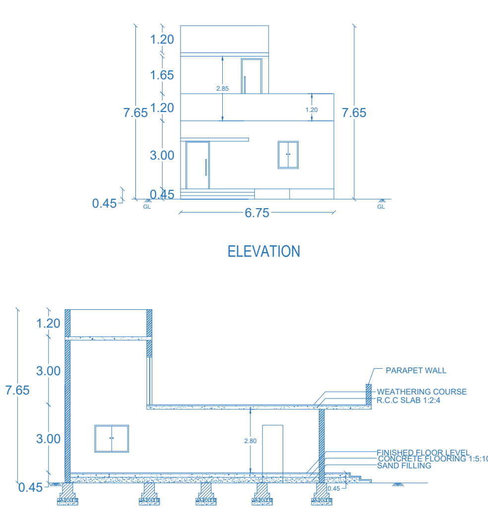
SECTION AA'
