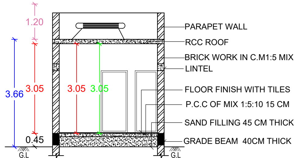
SECTION-AA1
