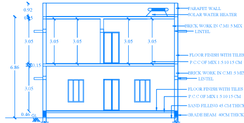
SECTION ON A-A1
