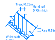
STAIR DETAILS
