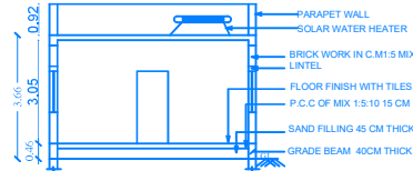
SECTION-AB
