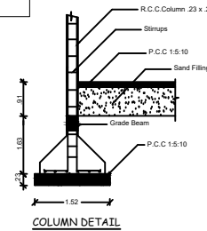
COLUMN DETAIL
