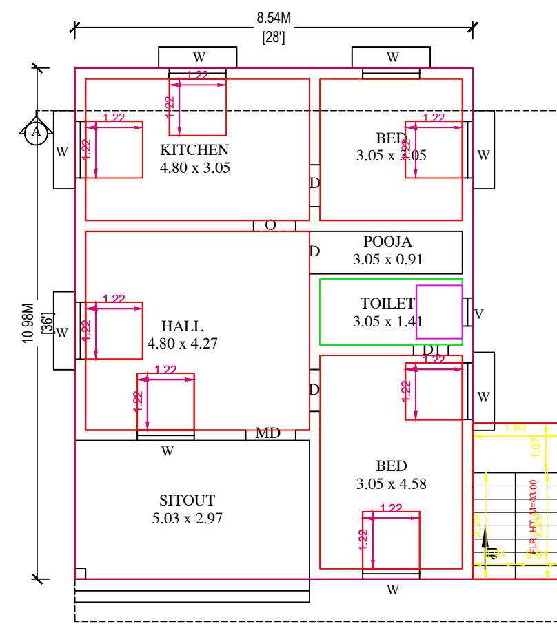
PRO.GOUND FLOOR PLAN
