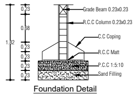
Foundation Detail
