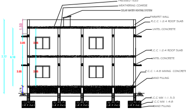
SECTION ON-"AA"
