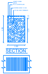
RAIN WATER HARVESTING PERCOLATION BED
