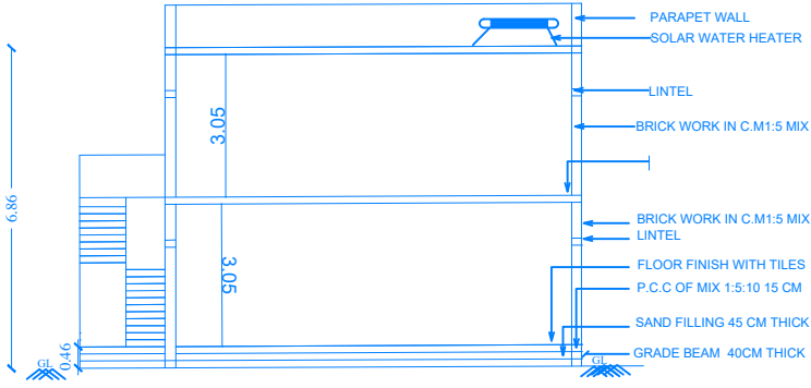
SECTION-AB
