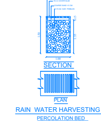
RAIN WATER HARVESTING PERCOLATION BED
